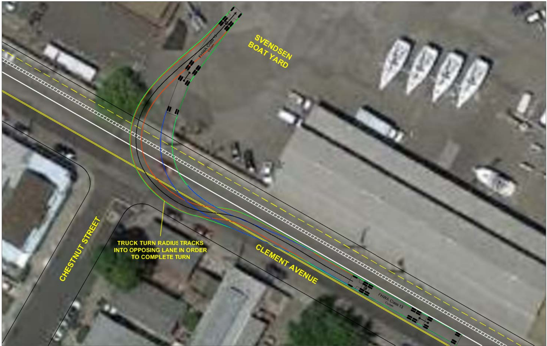
FHWA CLASS 13 TRUCK TURN CLEMENT AVENUE & CHESTNUT STREET ALAMEDA, CALIFORNIA
