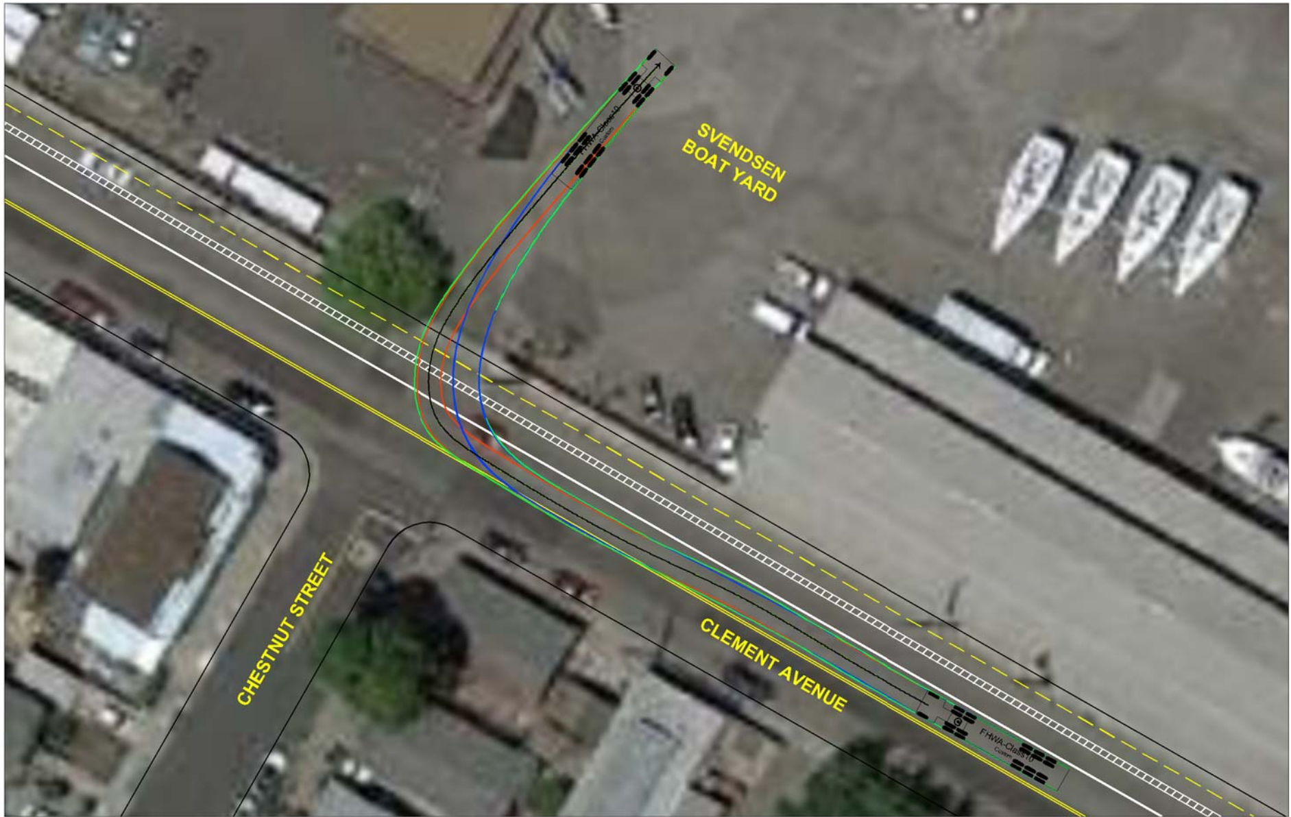
FHWA CLASS 10 TRUCK TURN CLEMENT AVENUE & CHESTNUT STREET ALAMEDA, CALIFORNIA
