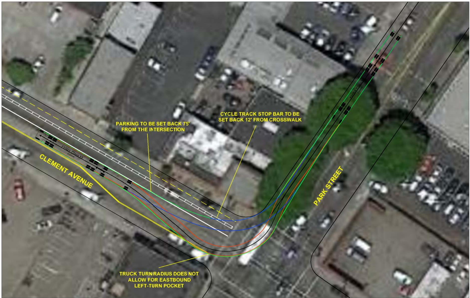
FHWA CLASS 13 TRUCK TURN CLEMENT AVENUE & PARK STREET ALAMEDA, CALIFORNIA
