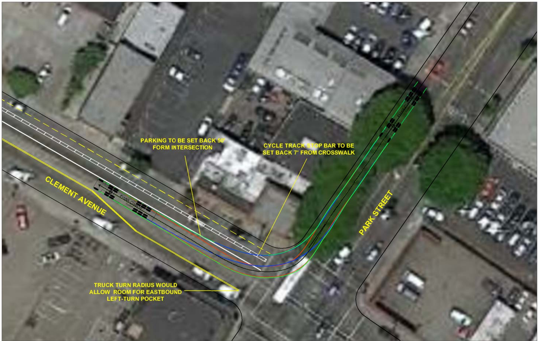
FHWA CLASS 10 TRUCK TURN CLEMENT AVENUE & PARK STREET ALAMEDA, CALIFORNIA
