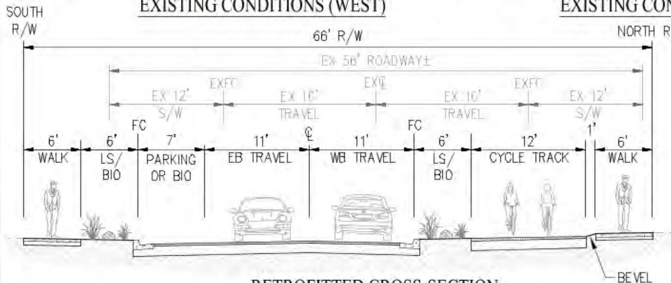
RETROFITTED CROSS-SECTION
