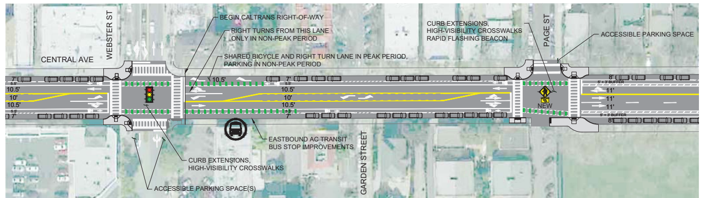
CLASS II BICYCLE LANE OPTION
