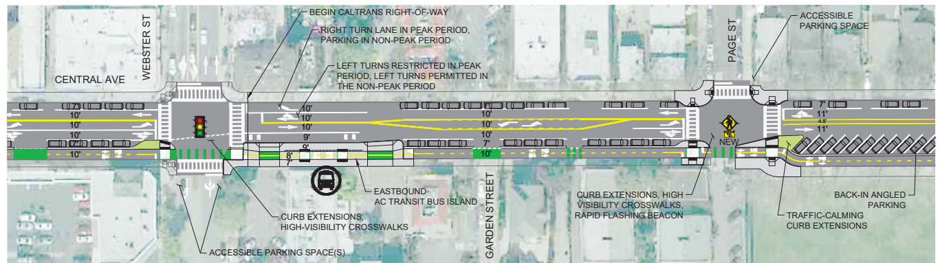
TWO-WAY PROTECTED BIKEWAY OPTION
